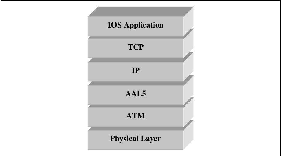
Figure 2.2-2 A3 and A7 Signaling Protocol Stack
