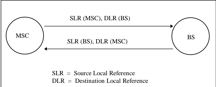
Figure 4.4.6-1 SLR/DLR Usage
