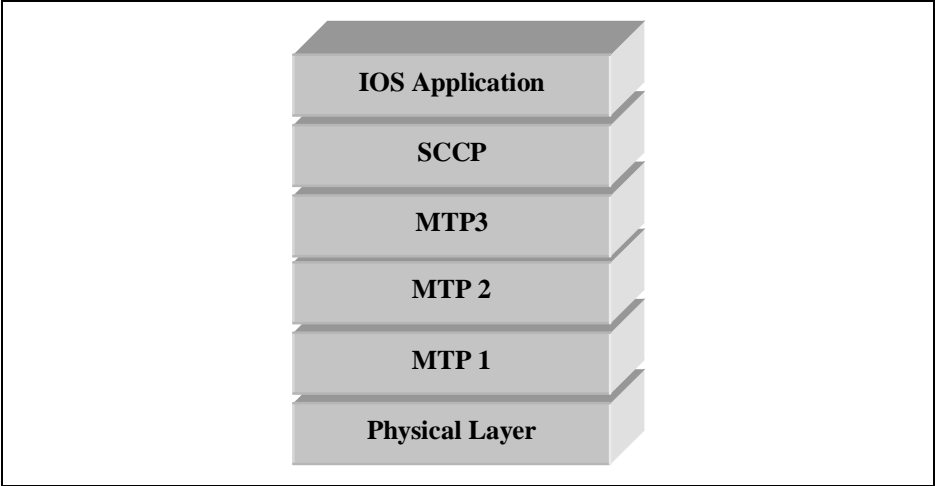
Figure 2.2-1 A1 Signaling Protocol Stack
