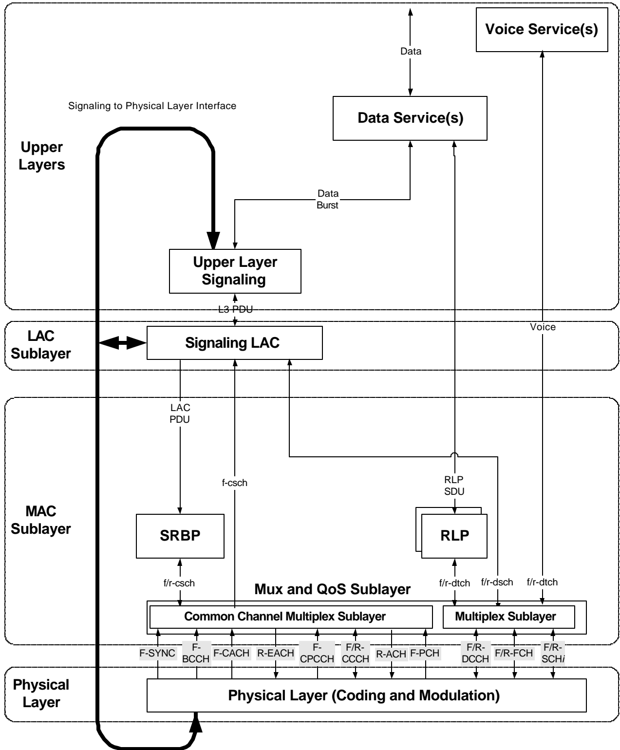
Figure 1. cdma2000 Architecture
