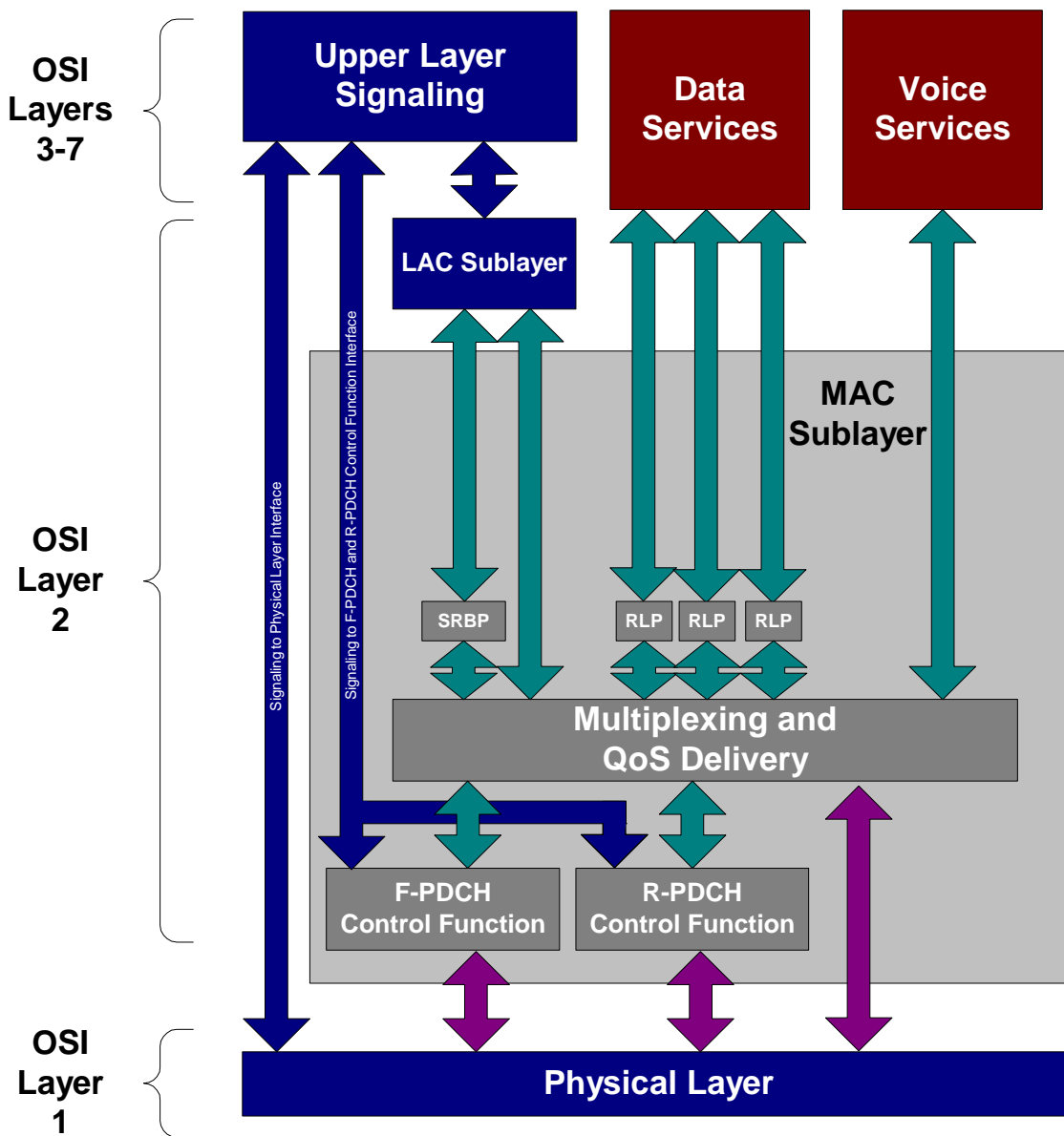
12 Figure 1 cdma2000 Architecture
